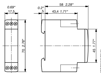
CT-C devices with 1 c/o contact or 2 n/o contacts
