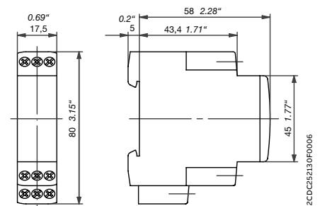
CT-C devices with 2 c/o contacts
