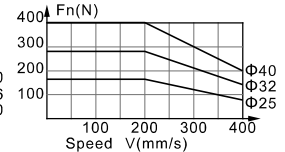
Force-Velocity chart (Pushing force in horizontal movement and moving velocity)
