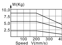
Load-Velocity chart (Load in vertical movement and moving velocity)
