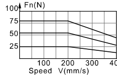
Force-Velocity chart (Pushing force in horizontal movement and moving velocity)
