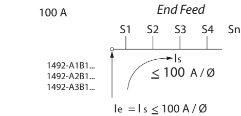
Figure 58 - Feeder Terminal and Bus Bar Current Distribution
