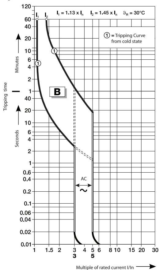
Figure 74 - B Curve
