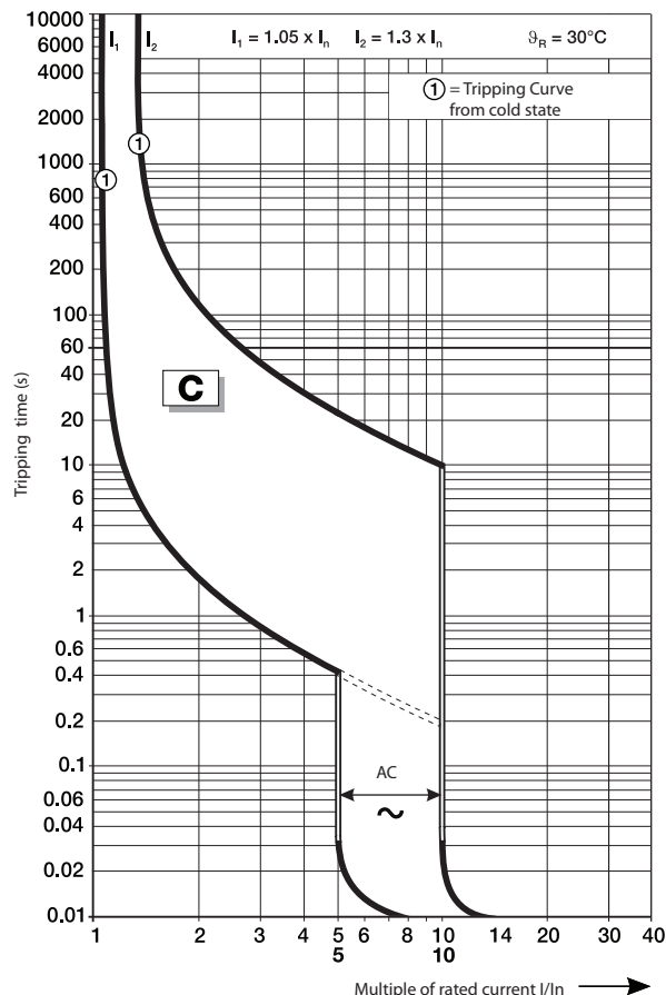
Figure 18 - C Curve
