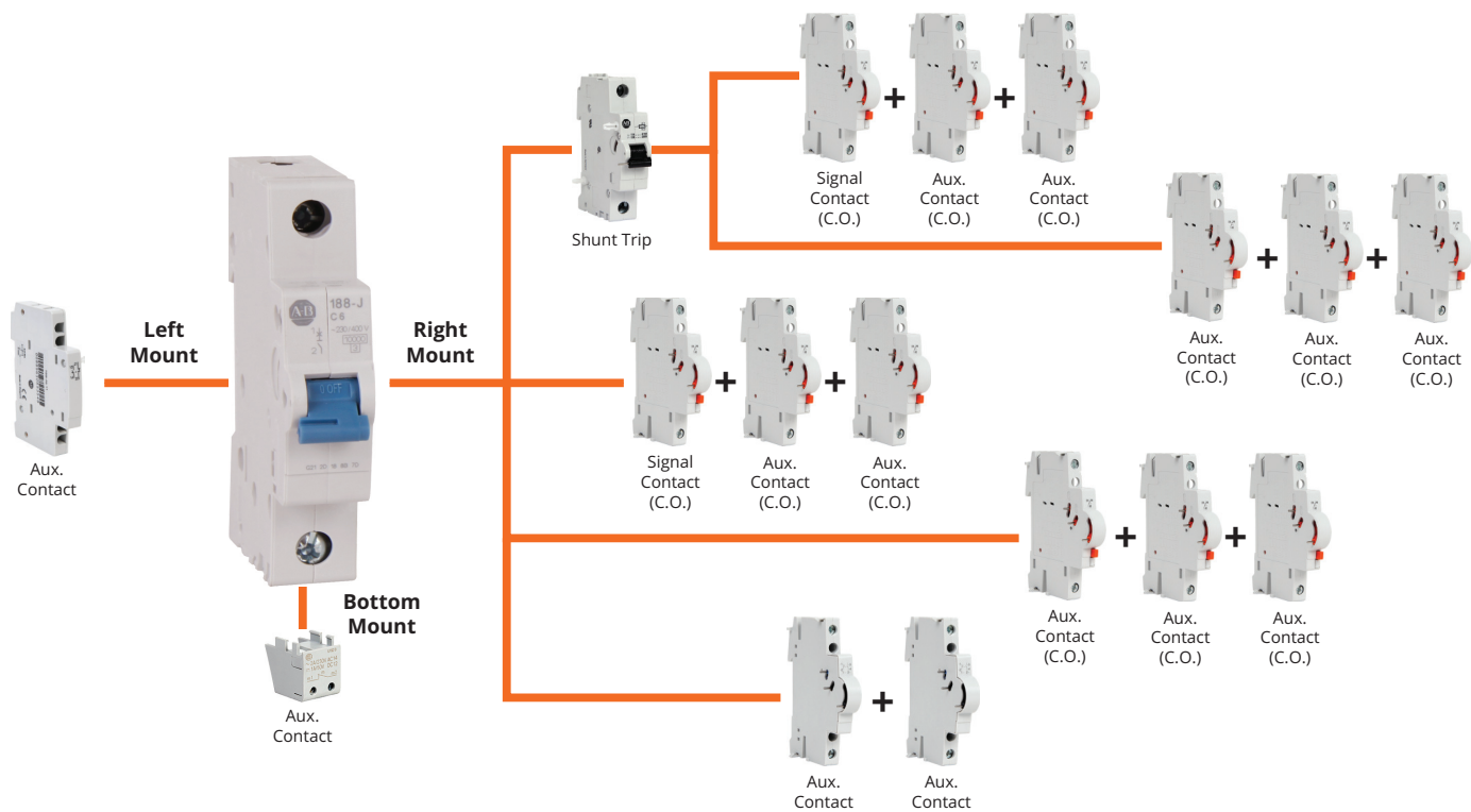
Figure 79 - Bulletin 188-J, -K Accessory Installation
