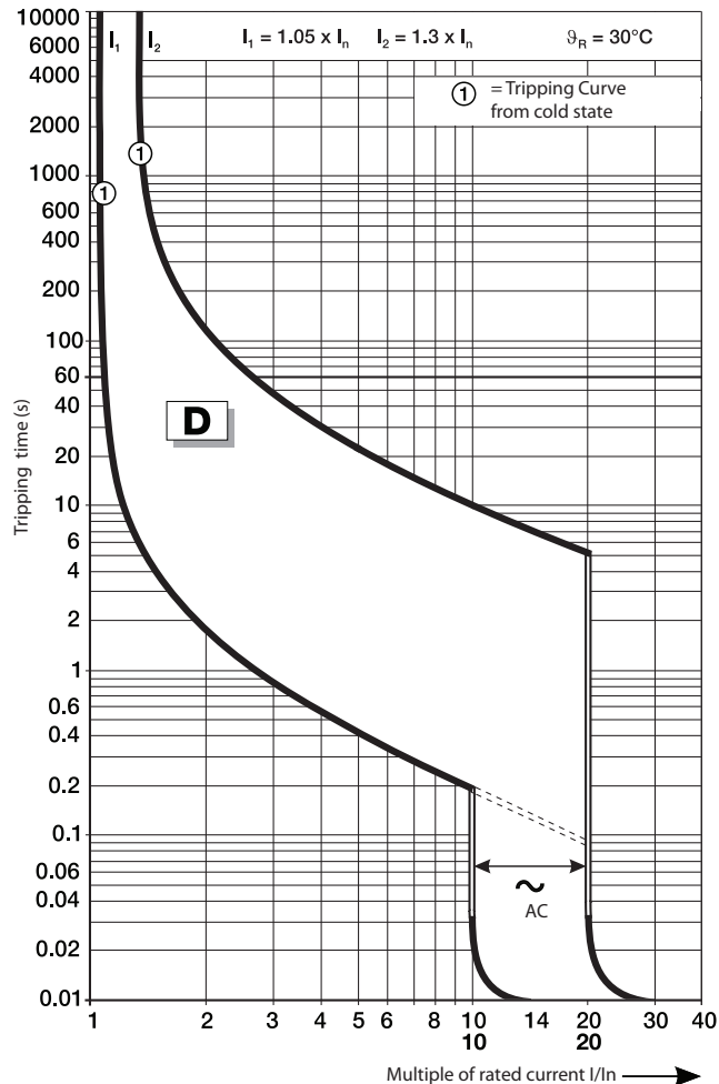
Figure 4 - D Curve
