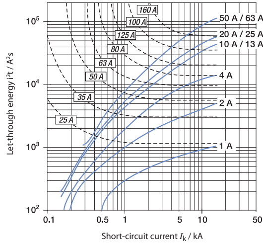
Figure 77 - D Curve
