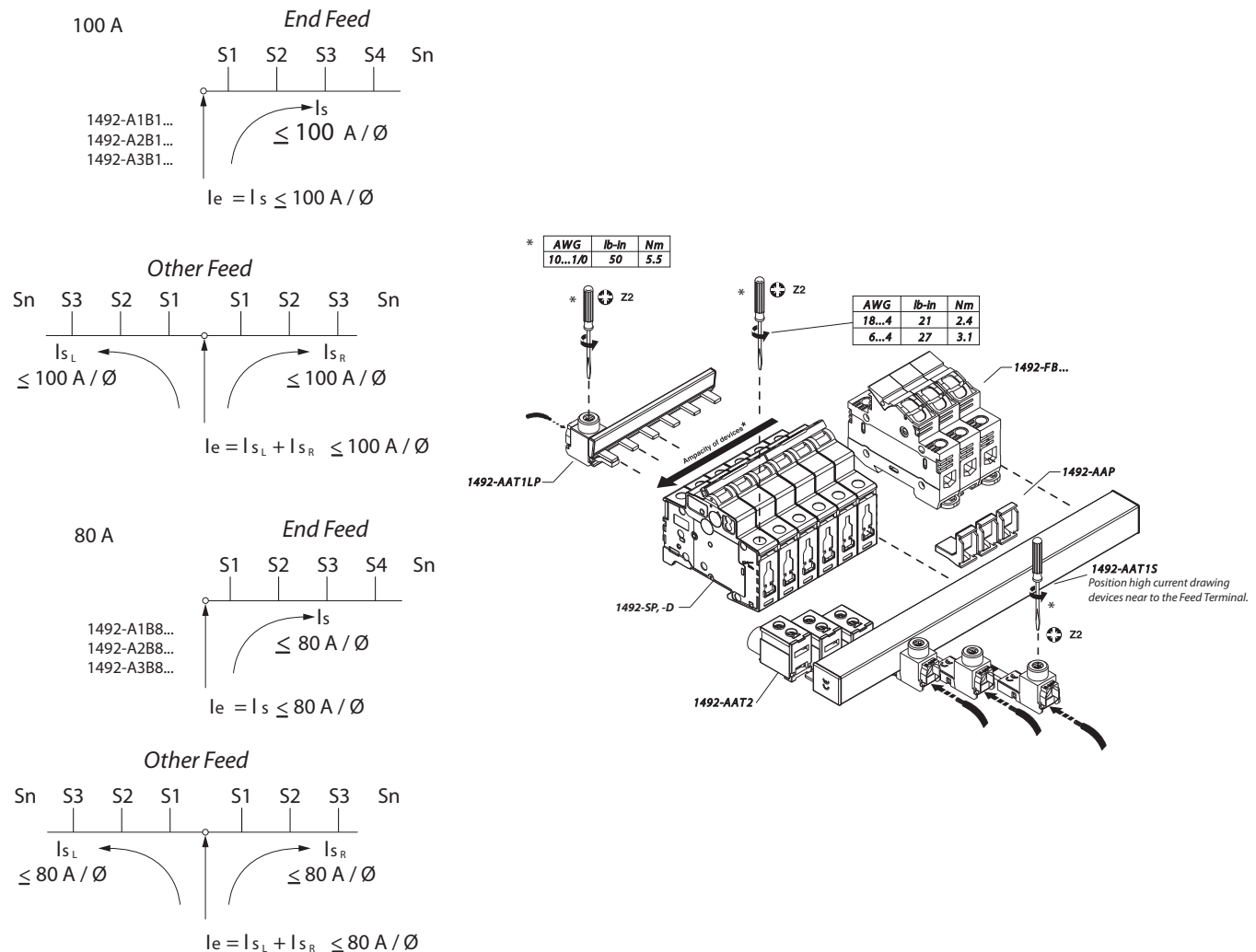
Figure 29 - Feeder Terminal and Bus Bar Current Distribution
