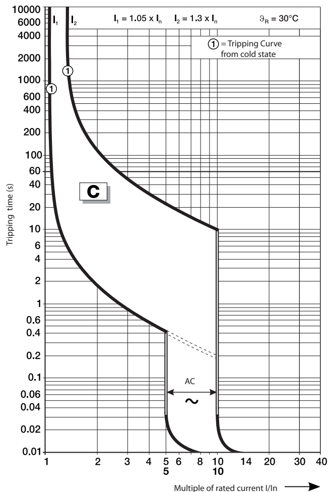
Figure 3 - C Curve
