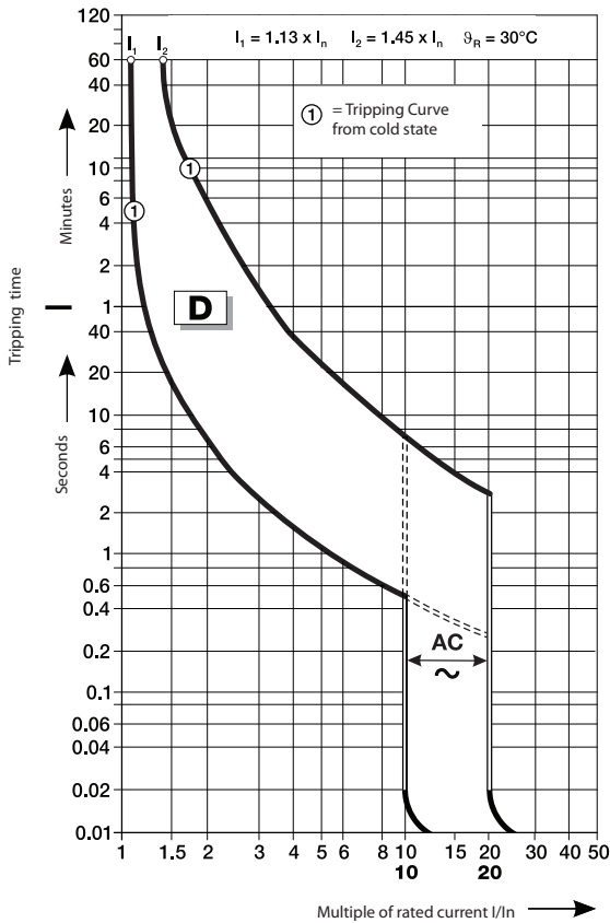
Figure 77 - D Curve
