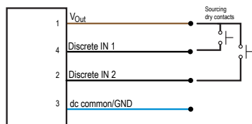
Figure 3. Wiring for dry contact mode
