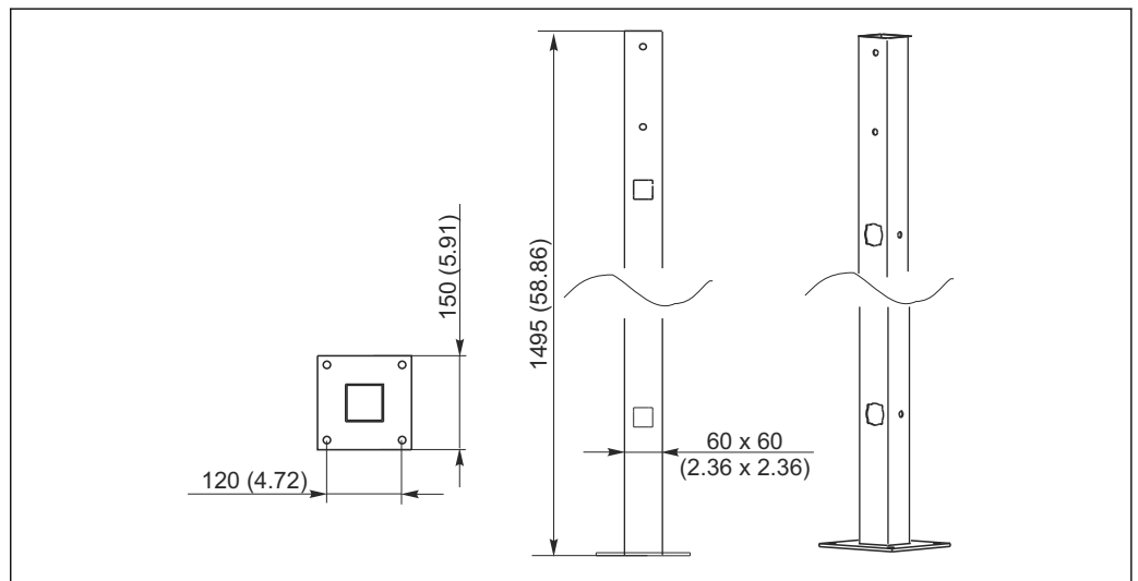
17 Dimensions in mm (inch)
