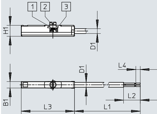
Dimensions – Proximity switch open end SDBC-MSB-1L-ZU-...
