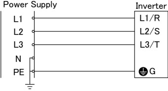
TN-S system
