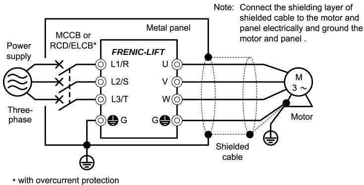
Figure 8.1 Installation inside a Panel
