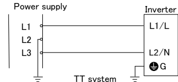
TT system (corner earthed/phase-earthed) (Applicable for 200V type only) *2)
