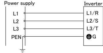
TN-C system
