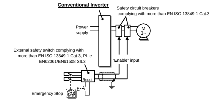
Figure 8.4 Conventional Inverters compliant with EN81-20 5.9.2.5.4 d) or EN81-20 5.9.3.4.2 d)
