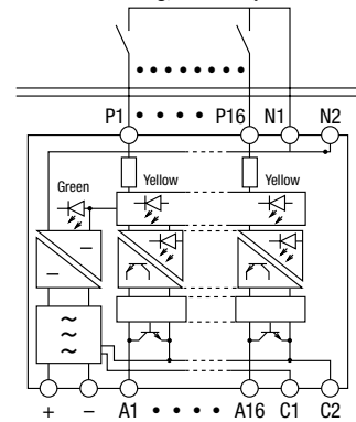
Connector Wiring, Sink Output
