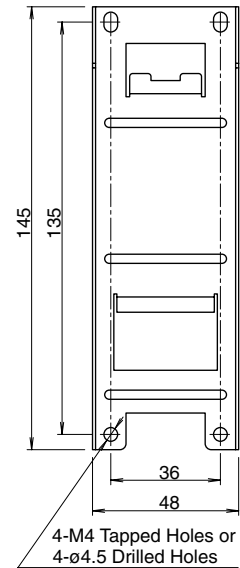
PS9Z-5R1G Panel Mounting Bracket
