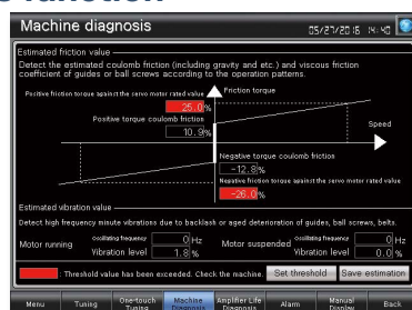
Machine diagnosis screen*
