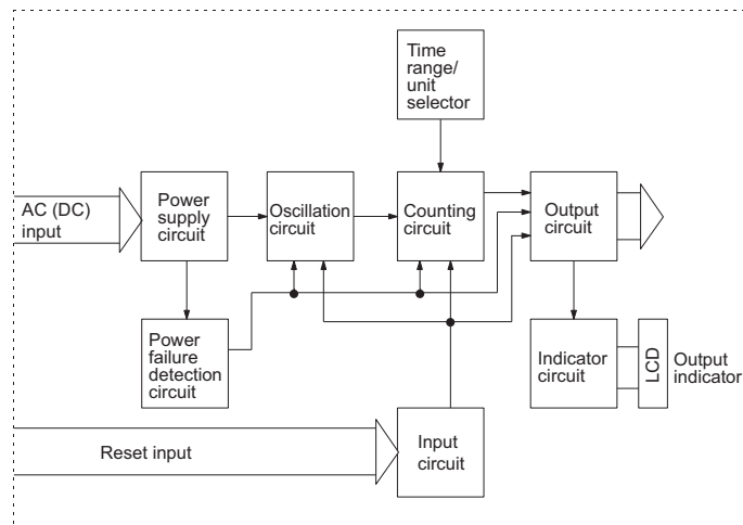
With Reset Input (H3CR-H8RL/-HRL)
