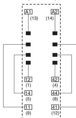
Terminal Arrangement/ Internal Connection Diagram (TOP VIEW)
