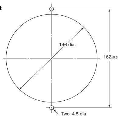
Outlet and Inlet
