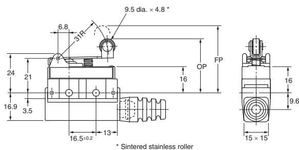
Short Hinge Roller Lever SHL-W255 SHL-W255-01
