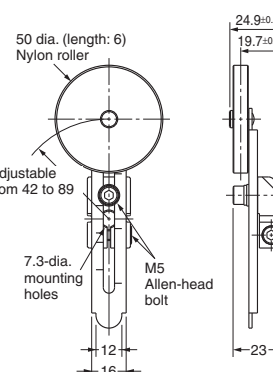
WL-2A104
