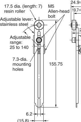
WL-2A104
