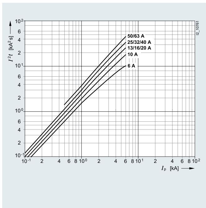
Characteristic B
