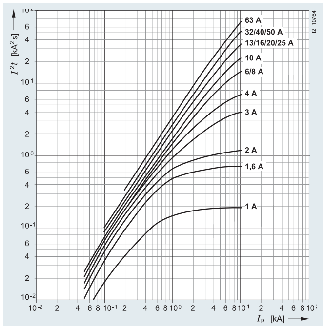
Characteristic A
