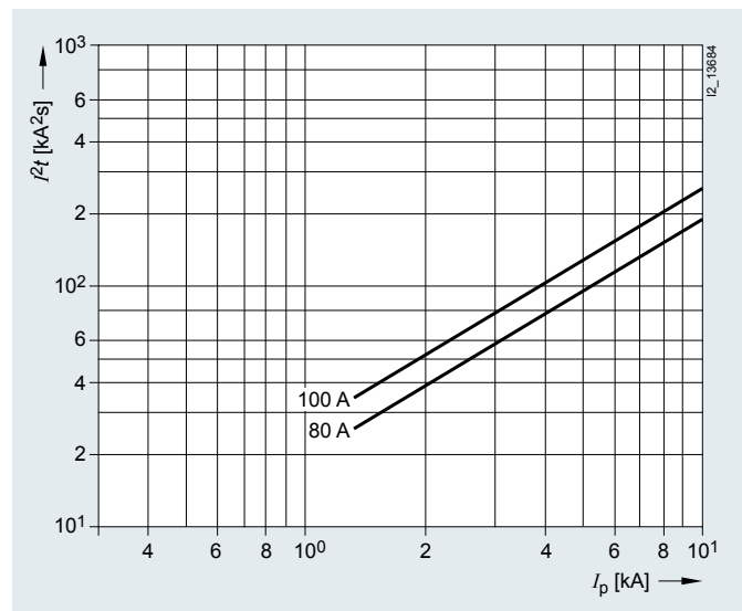
Characteristic D
