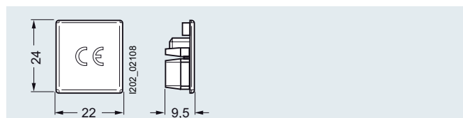
5ST3 750-0HG
