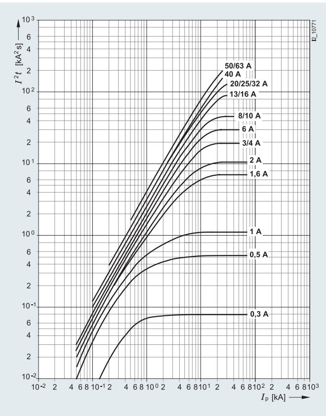
Characteristic C
