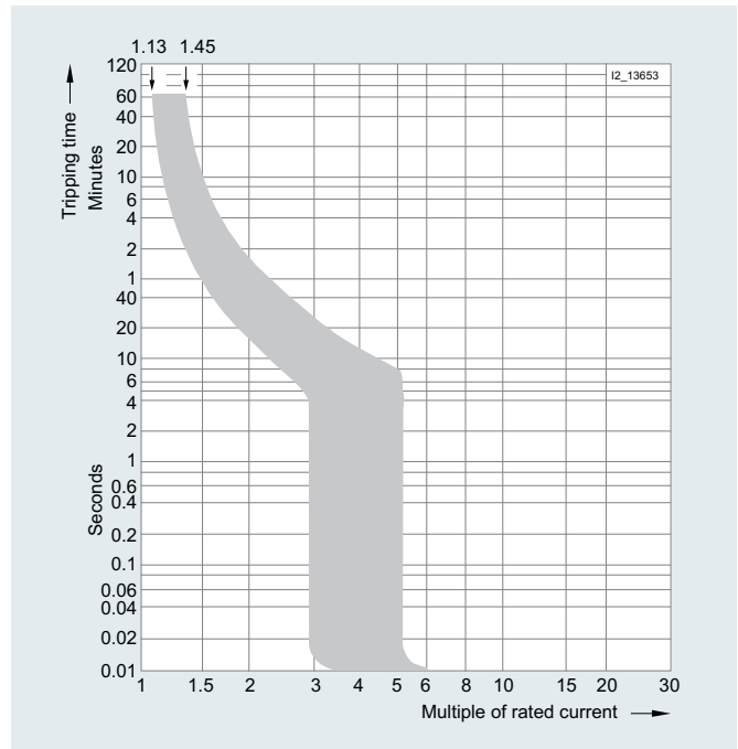
Tripping characteristic B
