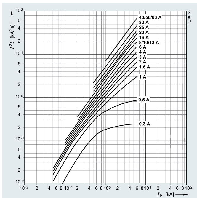
Characteristic D
