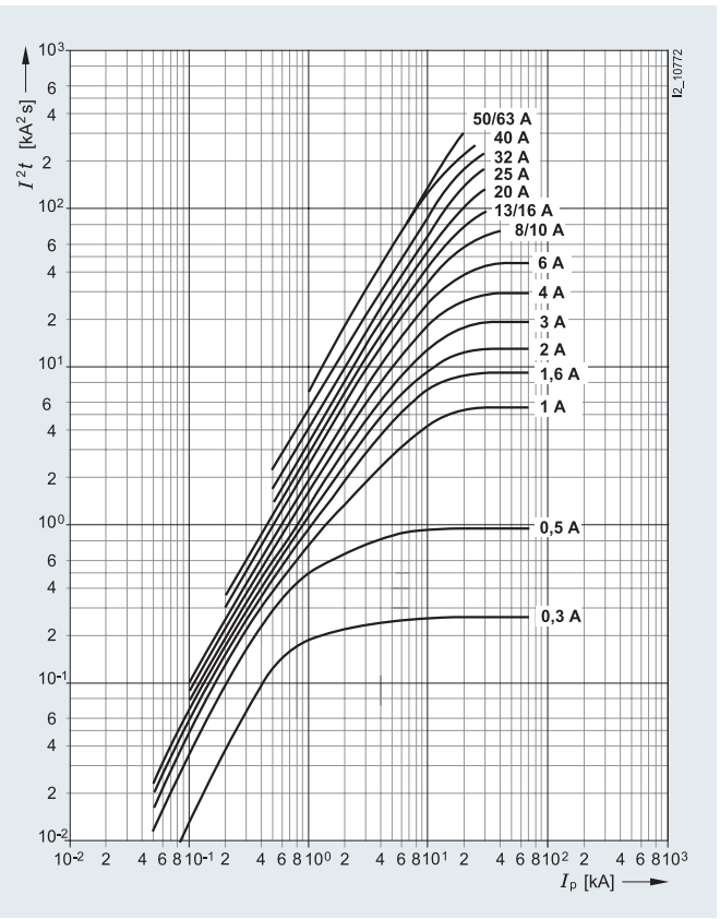
Characteristic D
