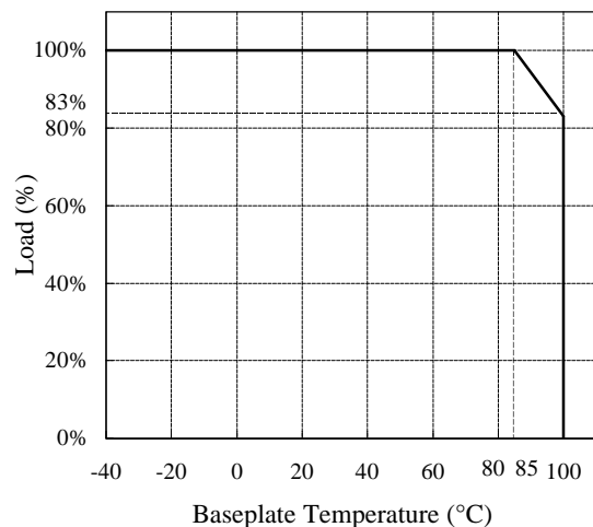
Derating Curve
